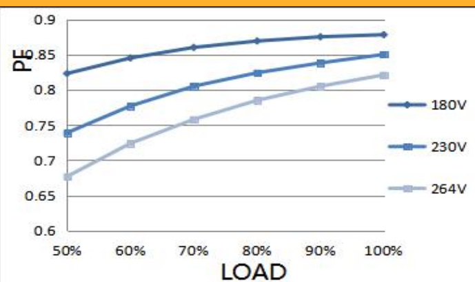
Fig.6 Efficiency-Load curve
