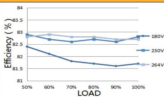
Fig.6 Efficiency-Load curve
